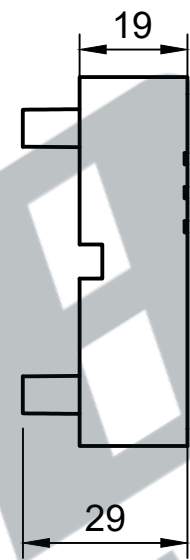
TOP (SIDE)
