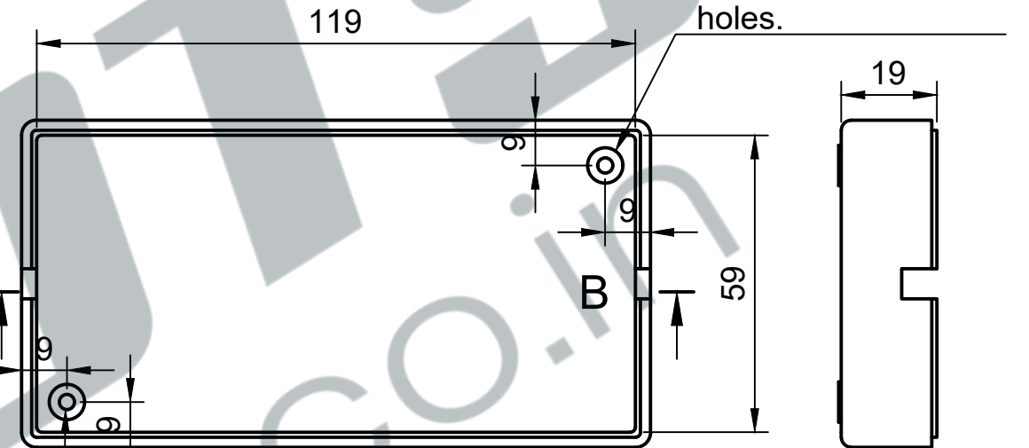
BOTTOM (SIDE)
