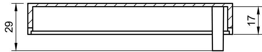
TOP (SECTION)
