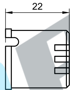
TOP(SIDE)
