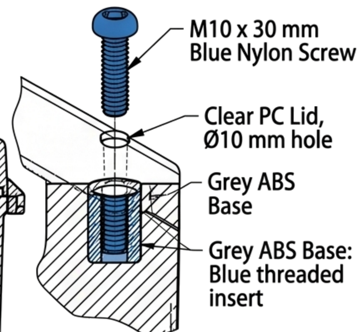
EXPLODED CORNER MTG
