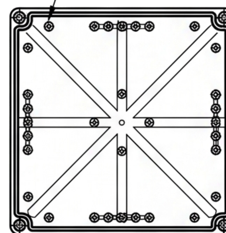
INTERNAL STANDOFF GRID (Top View)
