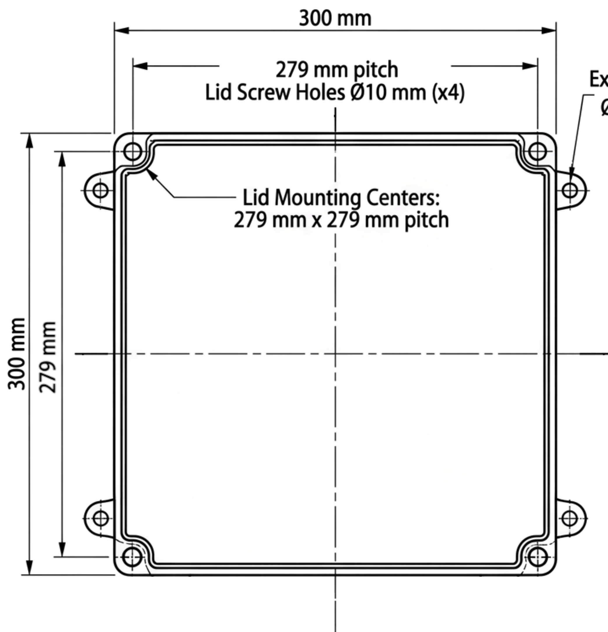
TOP VIEW (LID ON)
