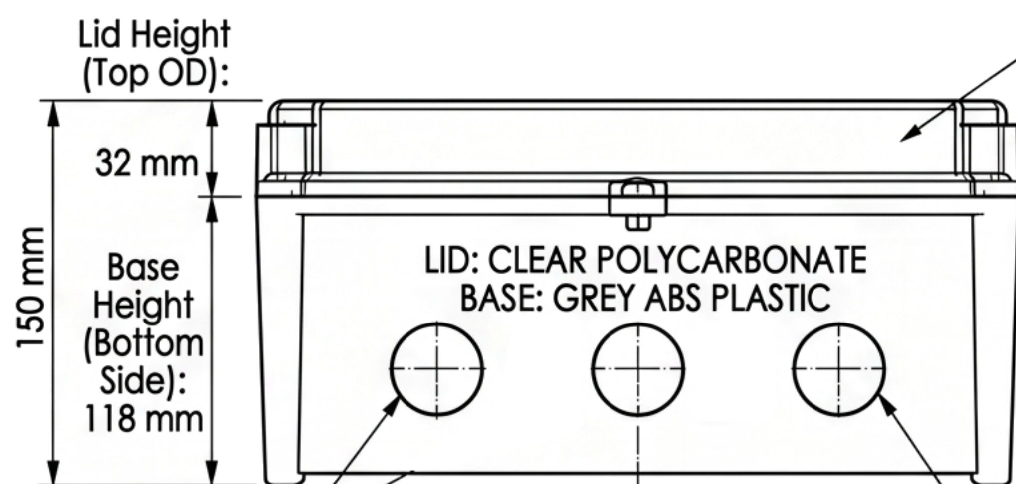
FRONT VIEW (CLOSED)
